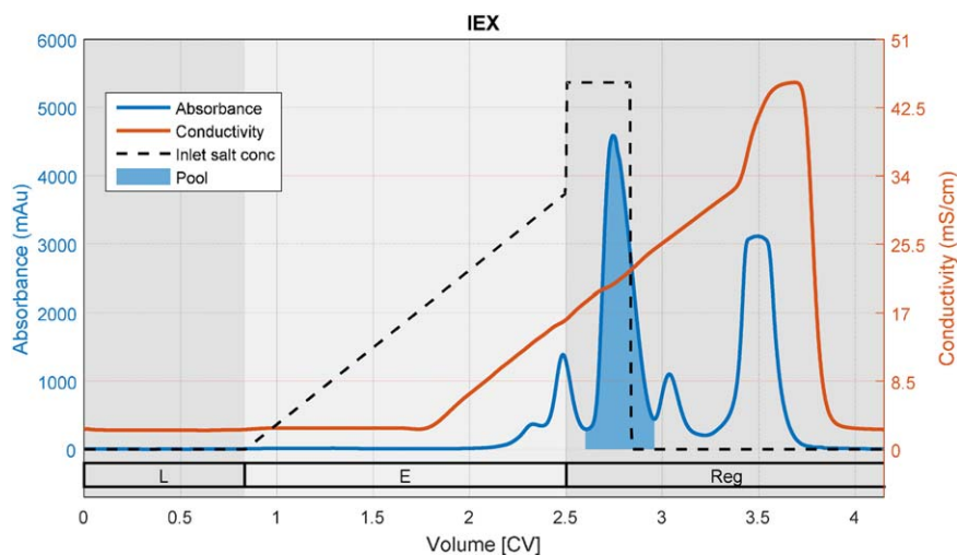
Figure 8. The chromatogram of the polishing step.
